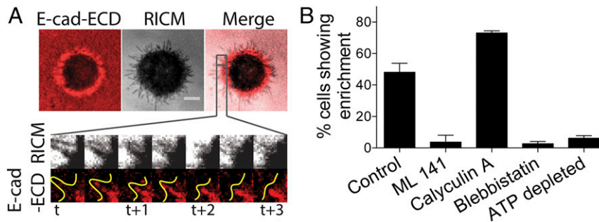
Fig. 4. E-cadherin clustering and junction formation is an actomyosin-dependent process. (A) Epifluorescence and RICM imaging of the cell shown in Fig. 2C revealing a tight contact with the bilayer around the zone of E-cad-ECD enrichment. Zoomed-in view of a retracting filopodia shows clustering of E-cad-ECD molecules. A trace of the retracting filopodia is overlapped on the epifluorescence image of E-cad-ECD on the bilayer. Numbers indicate time in minutes, with initial time assumed to be t . (B) Percentage of MKN28 cells, either untreated or treated with ML 141, calyculin A, blebbistatin, or a combination of antimycin A and 2'-deoxy glucose, showing enrichment of E-cad-ECD on partially fluid bilayers. Values represent mean \pm SD from multiple experiments. (Scale bar, 5 \mu m.)
